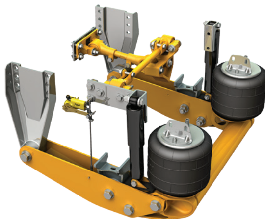
ADL and ADLSD Powered Suspension Models
