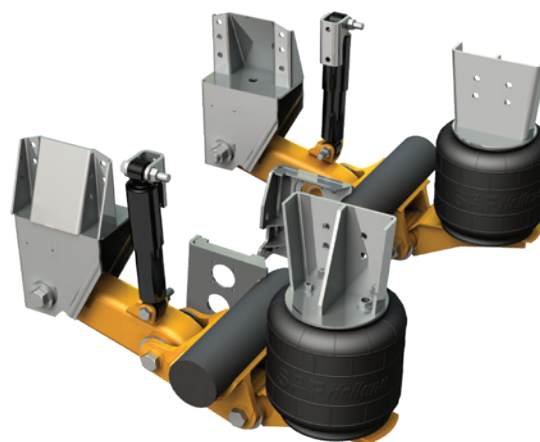
CA Suspension Models
