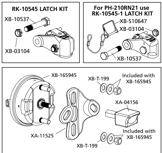
XA-02608 Cylinder and Bracket Sub-Assembly
